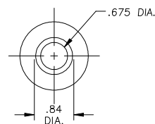
M-1331 MIXER SLEEVE FOR SULZER #ME-1324
