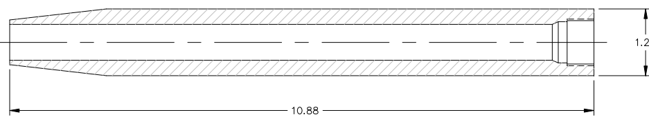
M-1580 MIXER SLEEVE FOR 161-224-W
