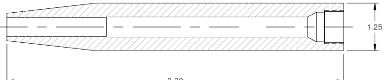
M-1582 MIXER SLEEVE FOR TAH #160-824-W TAH #160-824-AA-2
