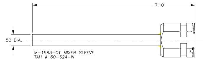
M-1583-QT MIXER SLEEVE TAH #160-624-W TAH #160-624-THIN TAH #160-624-THN/01 MIXER
