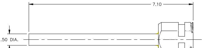
M-1583-QT MIXER SLEEVE TAH #160-624-W TAH #160-624-THIN TAH #160-624-THN/01 MIXER
