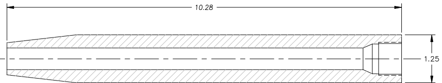
M-1333 MIXER SLEEVE FOR SULZER #MS-1324
