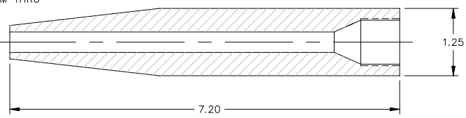
M-1583 MIXER SLEEVE FOR TAH #160-624-W TAH #160-624-THIN TAH #160-624-THN/01 MIXER
