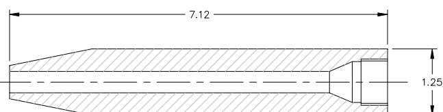
M-1101 MIXER SLEEVE FOR SULZER #ME-0624
