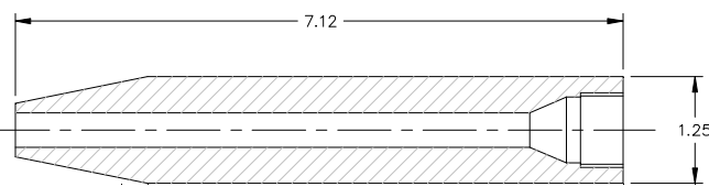
M-1101 MIXER SLEEVE FOR SULZER #ME-0624
