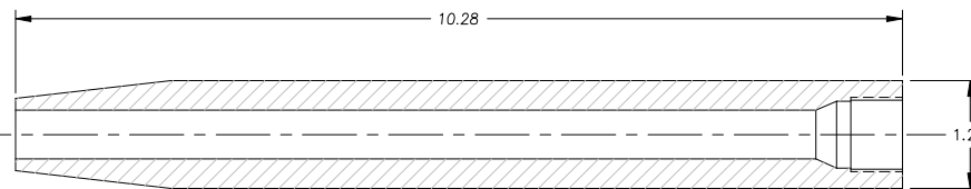
M-1333 MIXER SLEEVE FOR SULZER #MS-1324
