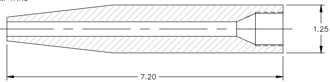
M-1583 MIXER SLEEVE FOR TAH #160-624-W TAH #160-624-THIN TAH #160-624-THN/01 MIXER
