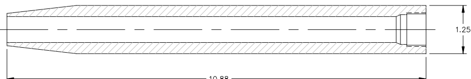
M-1580 MIXER SLEEVE FOR 161-224-W
