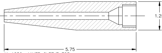
M-1852 MIXER SLEEVE FOR SULZER #ME-0524
