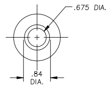
M-1331 MIXER SLEEVE FOR SULZER #ME-1324
