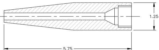
M-1852 MIXER SLEEVE FOR SULZER #ME-0524
